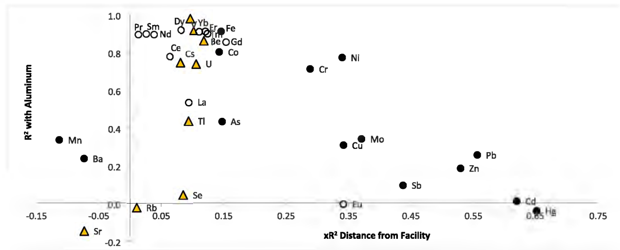
Fig. 3 Scatterplot of the strengths of each element's relationship to aluminum ( R^2 from linear regression) versus distance from the incinerator ( \times R^2 from nonparametric regression).
